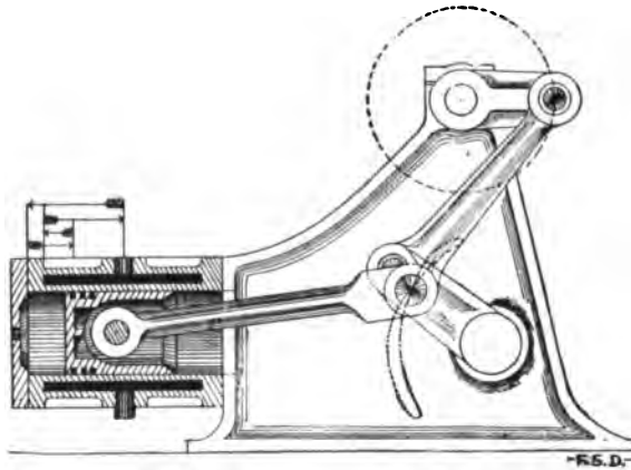
FIG. 304.—Section of the Atkinson Cycle Gas Engine, showing the varying lengths of the strokes—from the top, exhaust, expansion, compression, suction; also, the figure-of-8 path described by the toggle-jointed crank connections, and the path of the crank.
